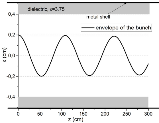
Fig. 4. The trajectory of the boundary bunch particle when emit_n = 0
